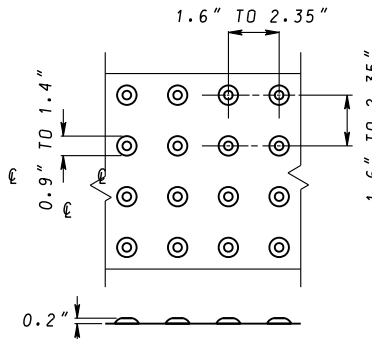
DOME SPACING
