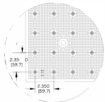
DETAIL A FIELD DOT 7 DOME LAYOUT
