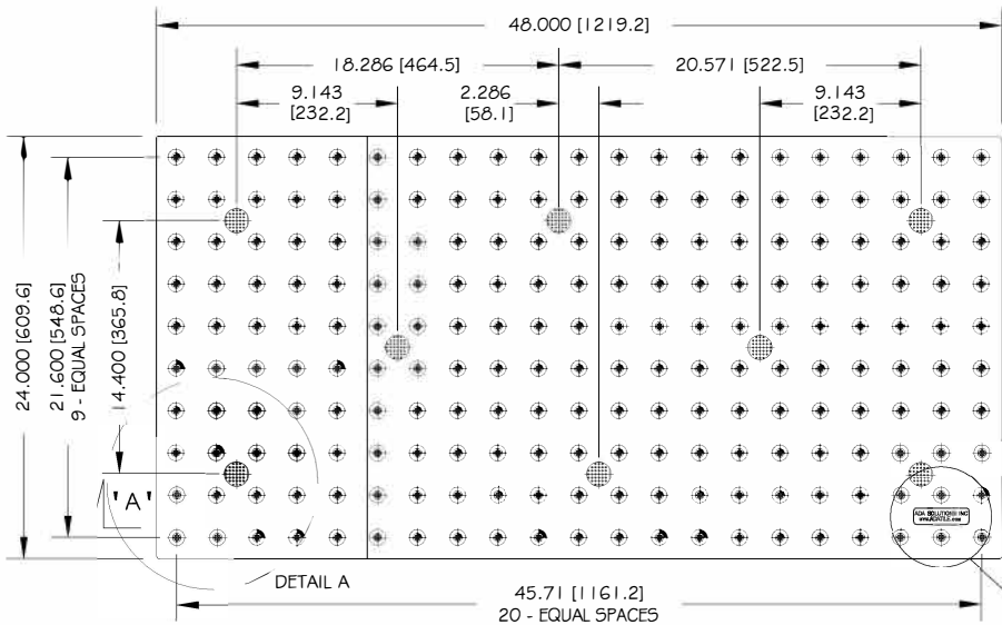
TOP OF PANEL
